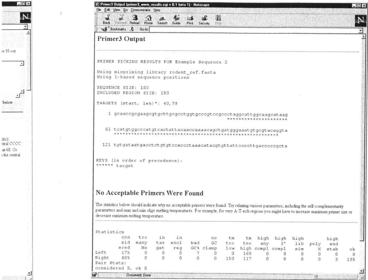
Fig. 6. Output from Primer3 's WWW interface when no primers were found.
